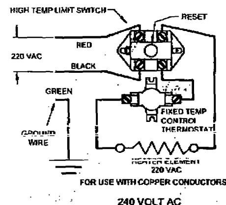
WIRING DIAGRAM FOR 240V
