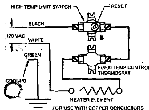
WIRING DIAGRAM FOR 120V
