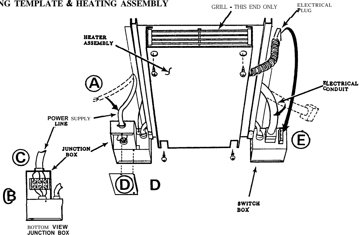
FIG. 8 CEILING TEMPLATE & HEATING ASSEMBLY
