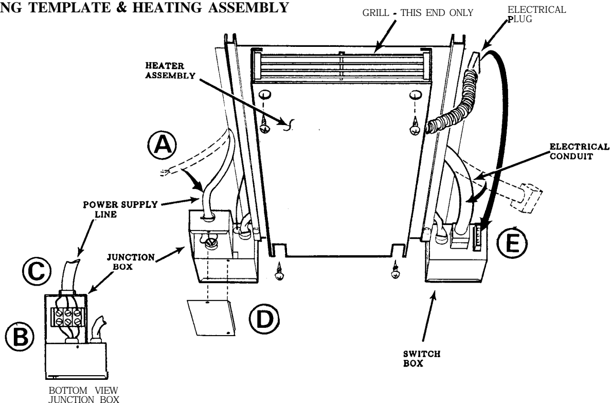
FIG. 8 CEILING TEMPLATE & HEATING ASSEMBLY
