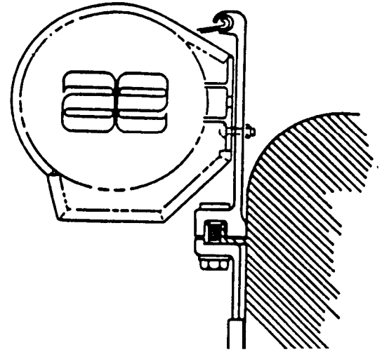
BRACKET ASSEMBLY FOR VAN INSTALLATION WITH OPTIONAL VAN ADAPTER BRACKETS (Kit No. 930035) (For permanent or temporary mounting onto rain gutters)
