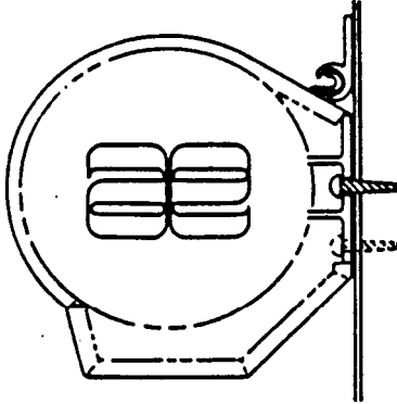
STANDARD FLAT MOUNT INSTALLATION WITH AWNING RAILS
