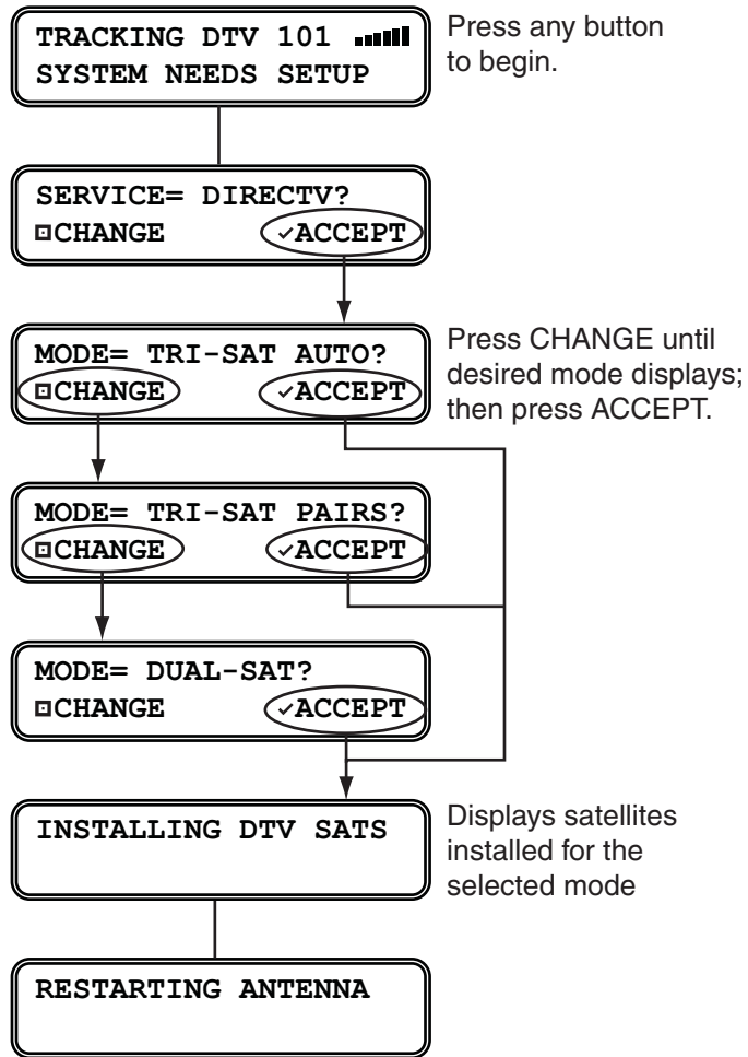
Figure 11 DIRECTV Setup
