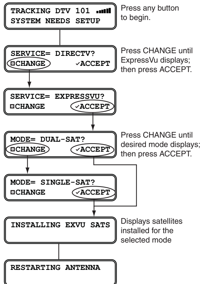
Figure 15 ExpressVu Setup
