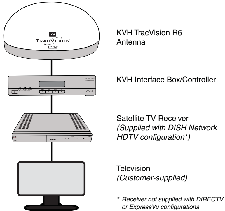
Figure 2 TracVision R6DX Basic System Diagram
