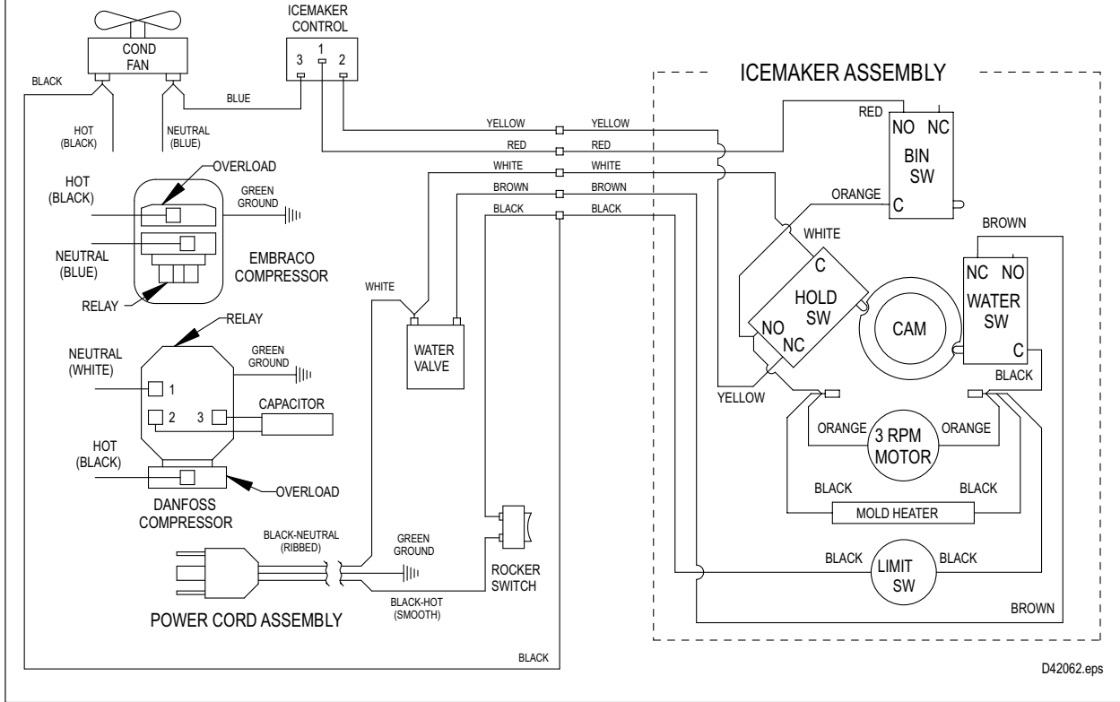
95, 98 AND SP18 WIRING DIAGRAM
