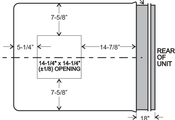
FIG. 1 AIR CONDITIONER DIMENSIONS (On Top of Vehicle) 579, 590, 591 & 595 SERIES
