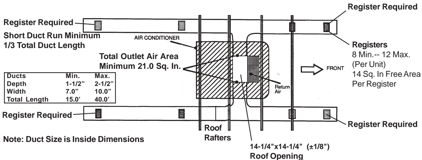
FIG. 32 Duct Size And Requirements For 33308120.XXX Genesis Air Filtration System Kit
