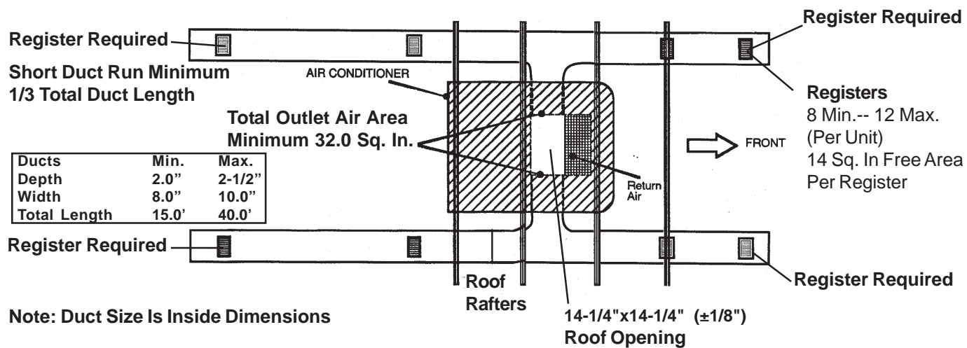
FIG. 32 Duct Size And Requirements For 33308120.XXX Genesis Air Filtration System Kit
