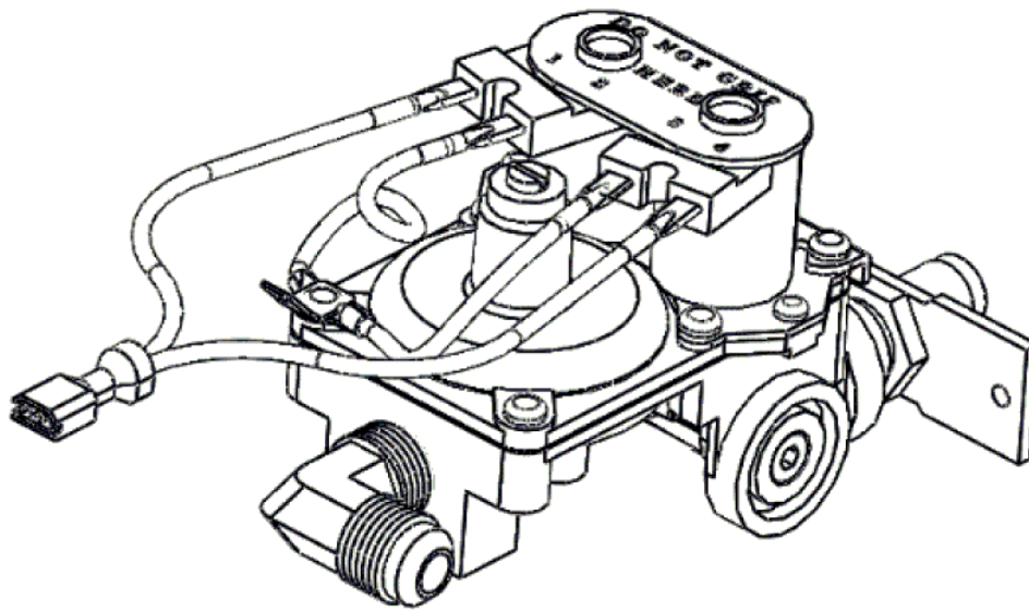
Valve Kit 31096
